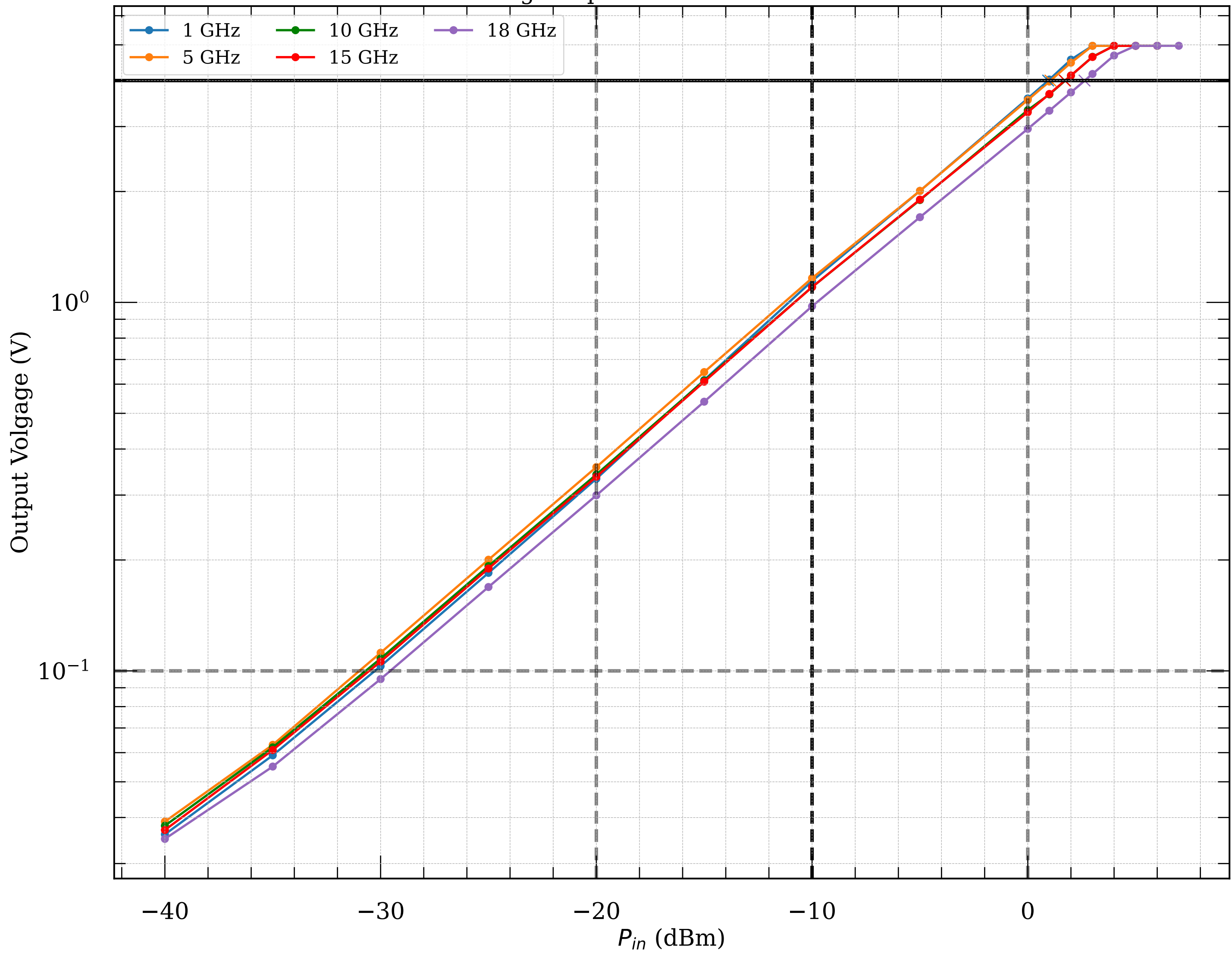
Measured voltage-to-power curve of detector module052
